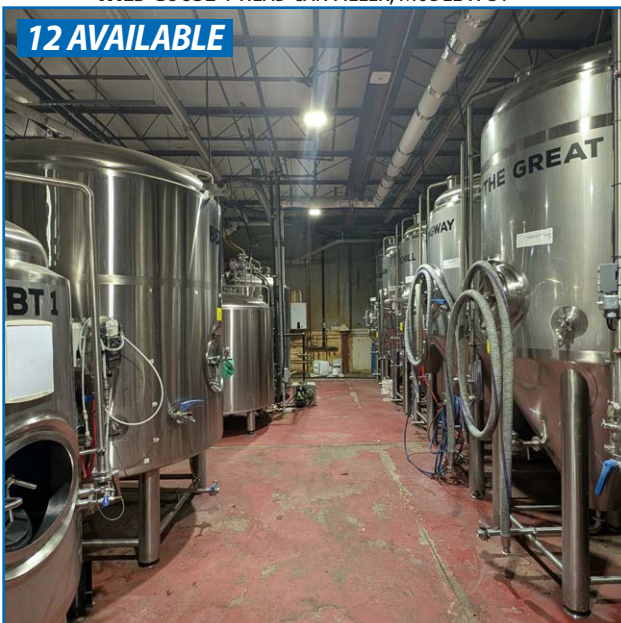
PARTIAL VIEW OF FERMENTATION VESSELS AND BRITE TANKS
