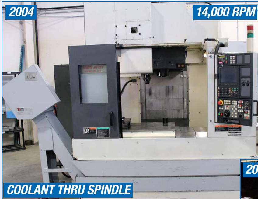
MORI-SEIKI NV5000 CNC VERTICAL MACHINING CENTER
