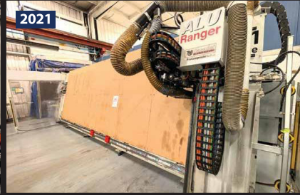
2021 CASADEI INDUSTRIAL ALU RANGER 6321 VG CNC VERTICAL PANEL ROUTER
