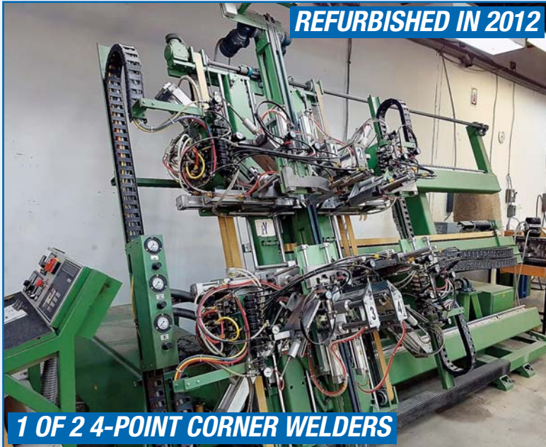
URBAN AKS 1400 ETL VERTICAL 4-POINT CORNER WELDER
