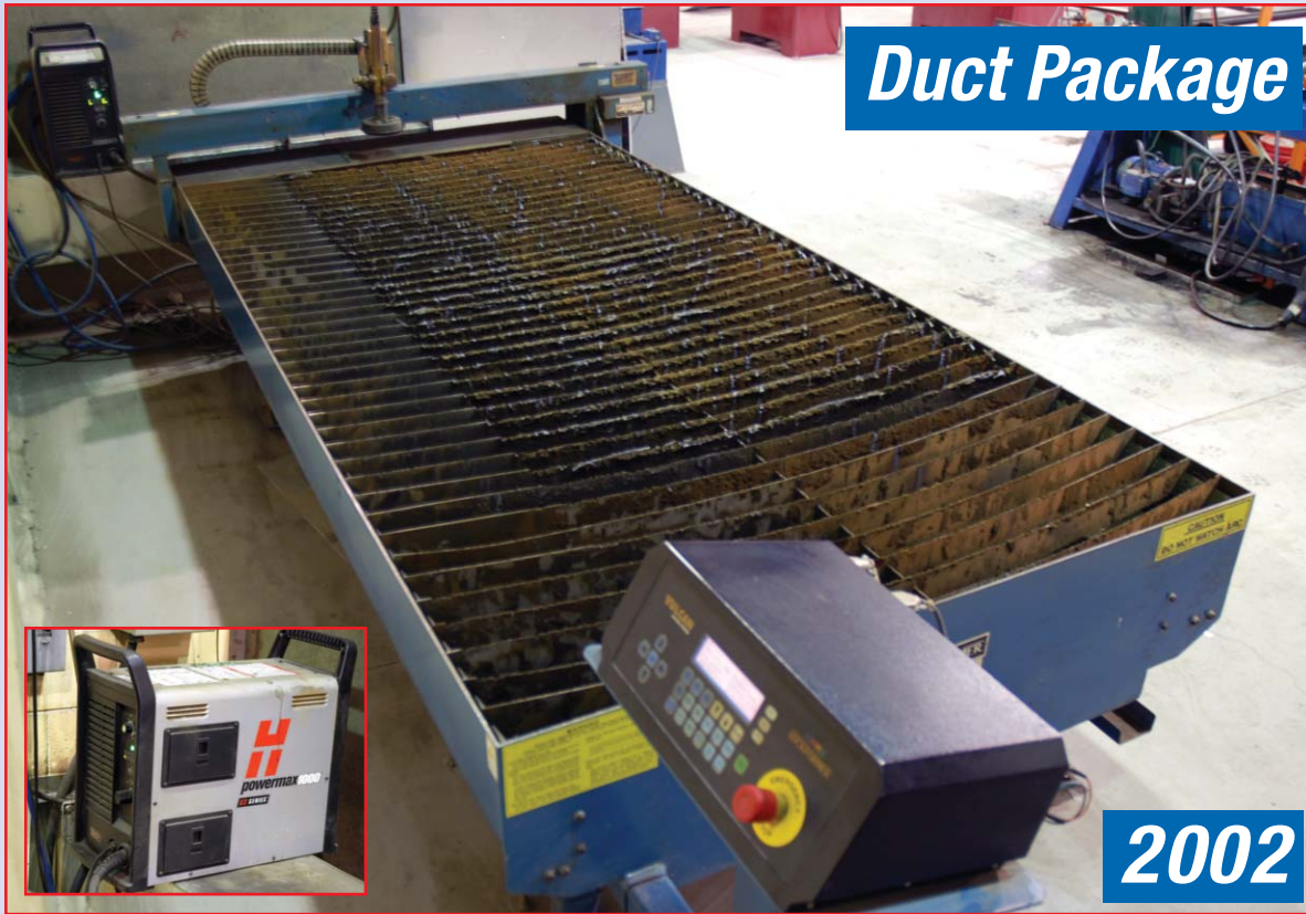
LOCKFORMER 5'X10' PLASMA CUTTER, MODEL VULCAN 1000
