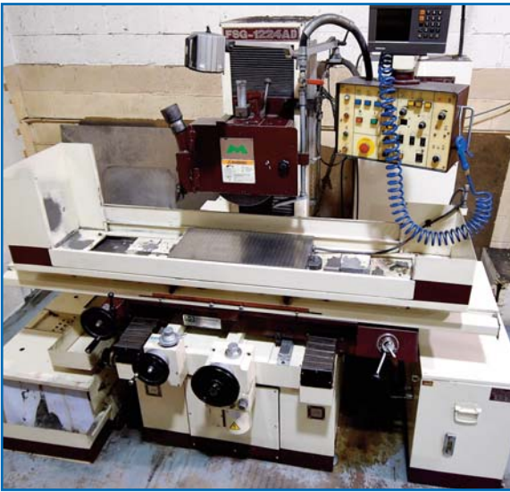
CHEVALIER FSG-1224AD AUTO HYDRAULIC SURFACE GRINDER
