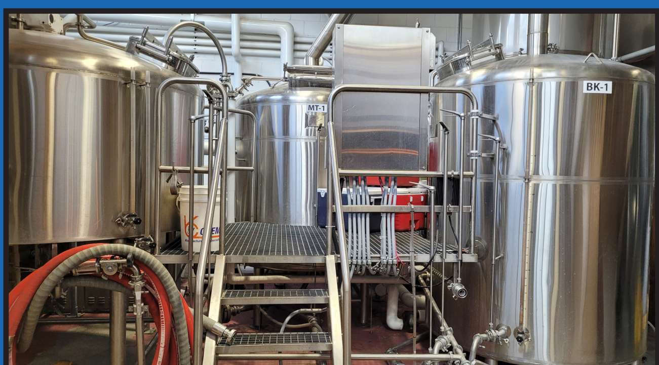
3-Vessel 20 HL Brewhouse consisting of: RIPLEY STAINLESS 20 HL C30 Mash Tun; RIPLEY STAINLESS Lauter Tun; Brewing Kettle; Hot Liquor Tank; (3) Pumps; ALFA LAVAL M6 Heat Exchanger; System Control Panel; Catwalk Structure
