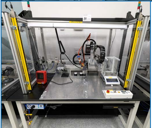
PARTIAL VIEW OF ROBOTIC HANDLERS, LEAK TESTERS & LAB CELLS
