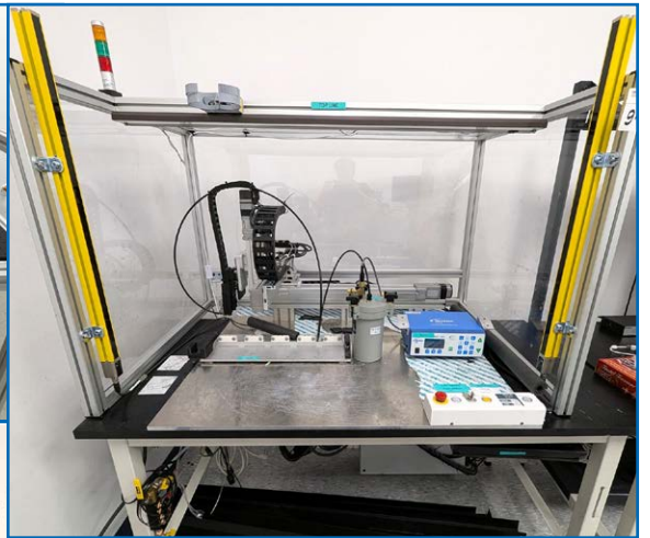
BALLERSTAEDT TWIN HEAT SEALER
