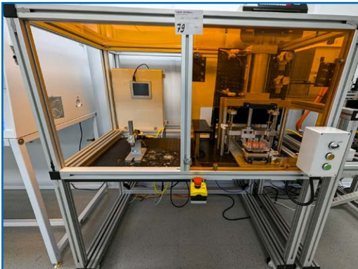
QVELLA FAST-PREP SYSTEM
