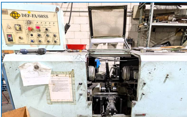
PARTIAL VIEW OF SOCO DOUBLE END TUBE CHAMFERING MACHINES
