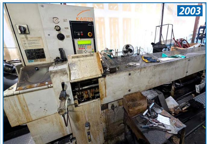
KASTO KASTOWA C7/9 CIRCULAR COLD SAW
