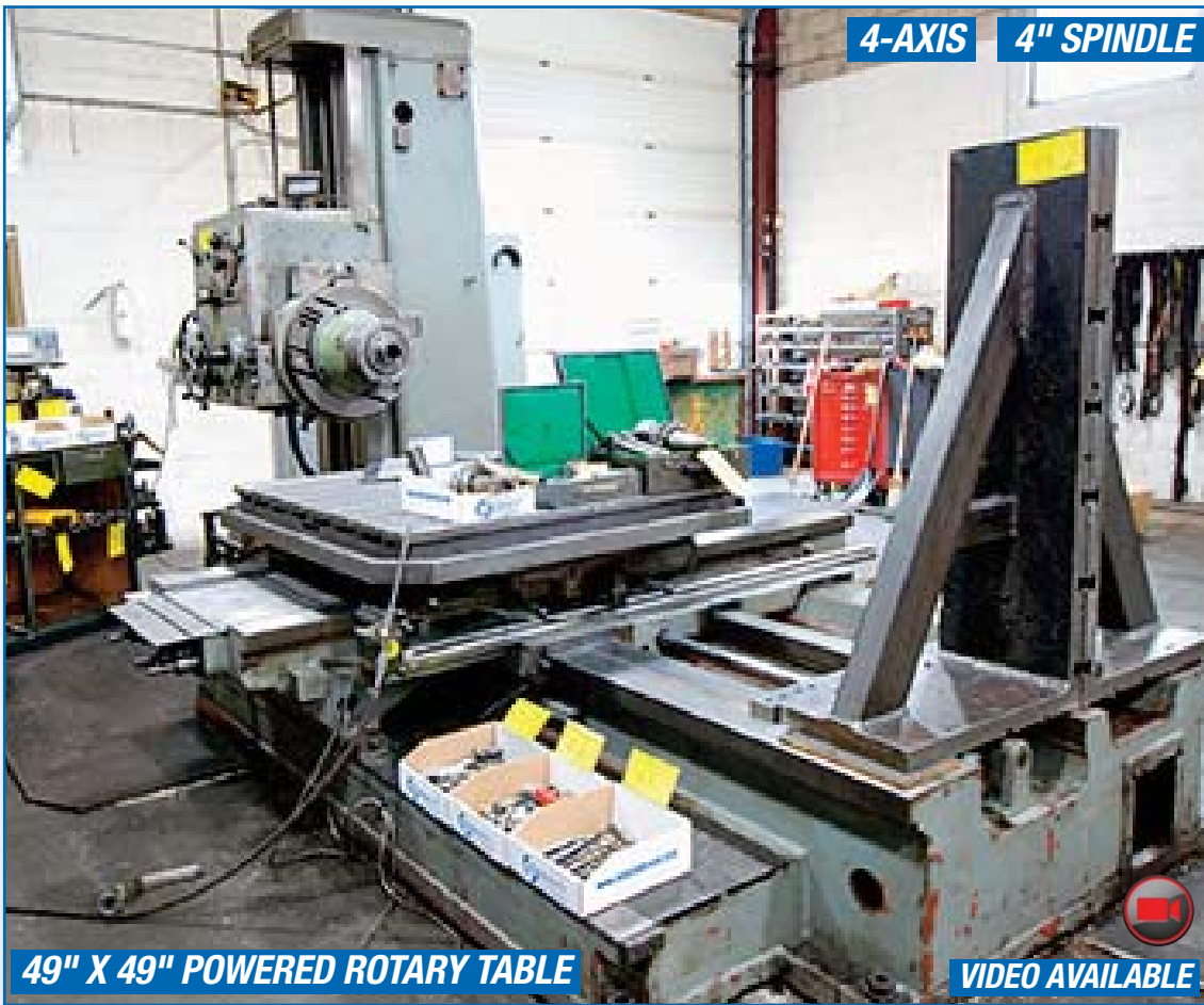
TOS W100 HORIZONTAL BORING MILL
