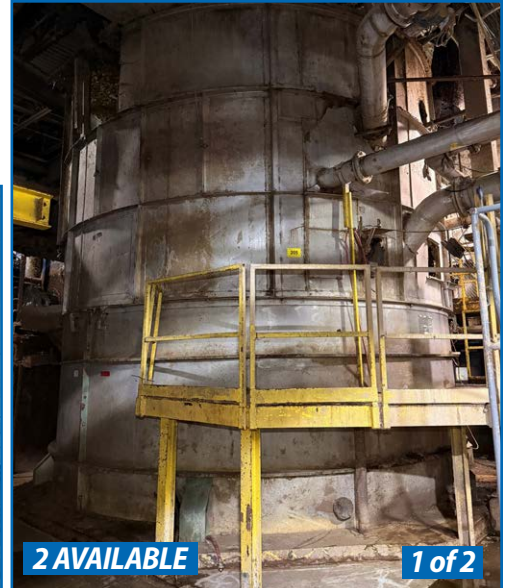
PULPERS 18', 20' DIAM PULPER. BLACK CLAWSON 700HP. CAPACITY TO PRODUCE 900TPD C/W OCC DETHRASHING SYSTEM
