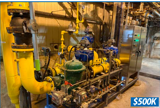
ARCTIC COMBUSTION RMS SYSTEM FUEL TRAIN
