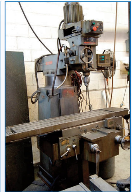
TOS FNK 25 VERTICAL MILLING MACHINE
