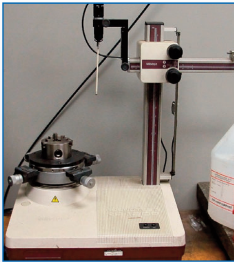
MITUTOYO RA-120P COMPACT ROUNDNESS MEASUREMENT SYSTEM
