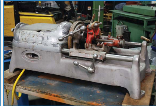
RIDGID MODEL 535 PIPE THREADER
