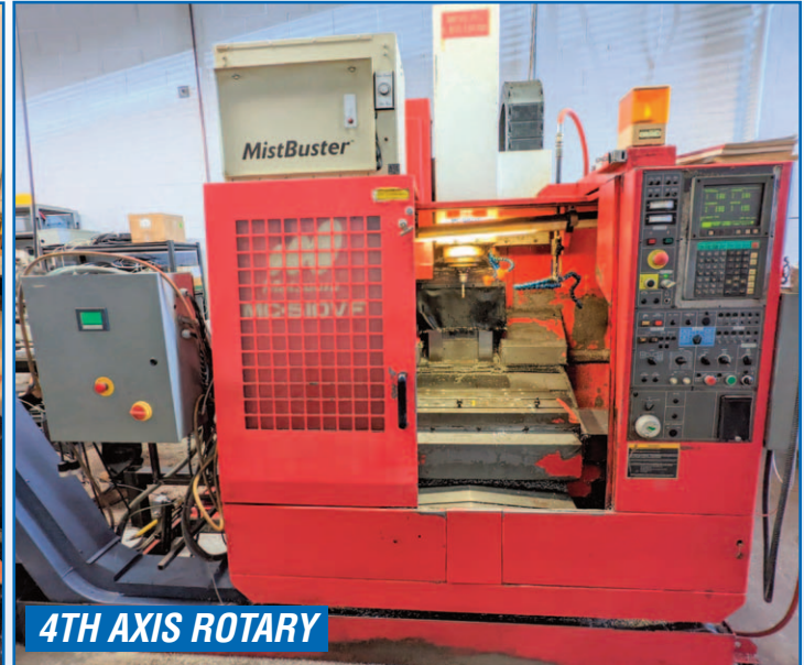
MATSUURA MC-510VF CNC VERTICAL MACHINING CENTER
