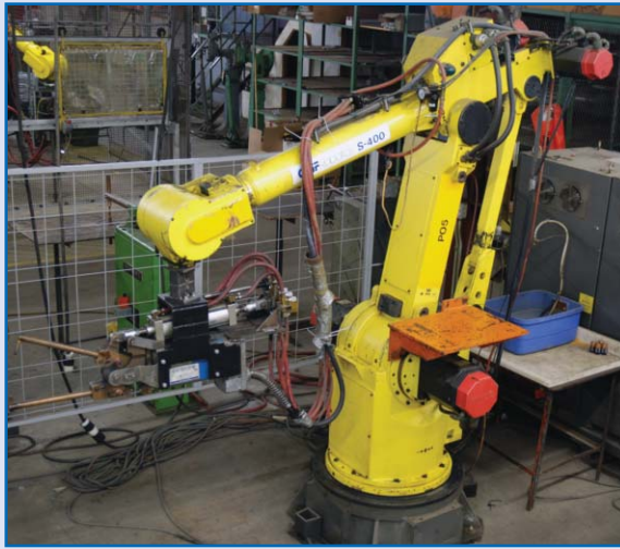
GMF S-400 6 AXIS ROBOTIC CELL, INCLUDING: MEDAR DIGITAL CONTROL PORTABLE SPOT WELDER (#8)
