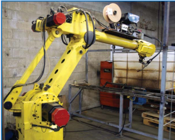
GMF S-400 6 AXIS ROBOTIC CELL, INCLUDING: COMPACOMATIC WELDER (#4)
