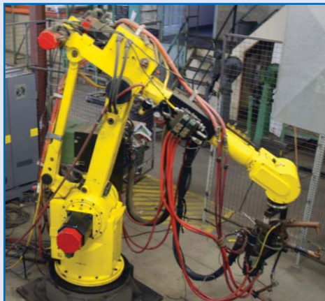
GMF S-400 6 AXIS ROBOTIC CELL, INCLUDING: MILLER MAXTRON 450 WELDER (#7)
