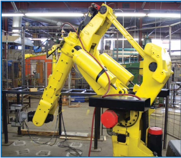
FANUC S-420iF 6 AXIS ROBOTIC CELL, INCLUDING: PRECISION 100 KVA & PEER 50 KVA SPOT WELDERS (#1)
