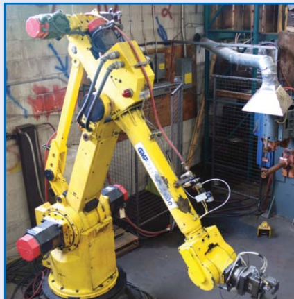
GMF S-400 6 AXIS ROBOTIC CELL, INCLUDING: COMPACOMATIC WELDER (#4)
