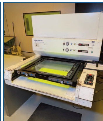
ORC MODEL HMW 201 B AUTOMATED EXPOSURE UNIT
