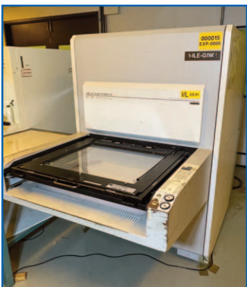
OLEC ACCUPRINT MODEL AP30-5000 POWER PLUS 5KW HIGH RESOLUTION DOUBLE SIDED VACUUM EXPOSURE
