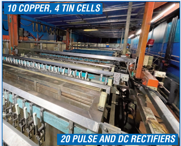
PAL AUTOMATIC CIRCUIT BOARD PLATING LINE
