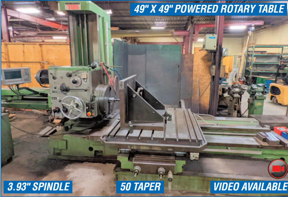
TOS W100A HORIZONTAL BORING MILL
